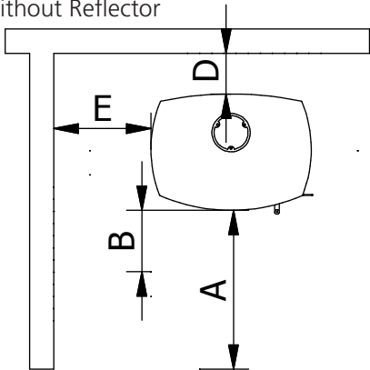
Without Reflector
