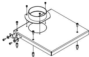
8381790 Air-box
