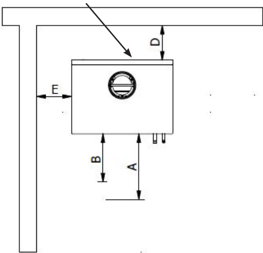
With Reflector
